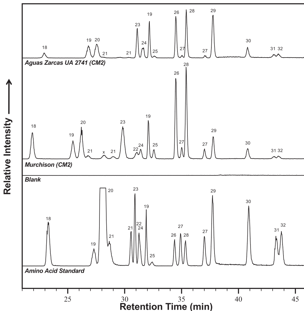
Fig. 2. The 21–46 min. region of the LC-Q-ToF-MS single ion chromatograms of the C 5 amino acids ( m/z = 379.1328 \pm 10 ppm). o -phthalaldehyde/ N -acetyl-L-cysteine derivatization (15 min) of amino acids in the standard and of the 6 M HCl-hydrolyzed, hot-water extracts of the procedural blank and the CM2 Murchison (Chicago Field Museum, 1.0 g extract) and Aguas Zarcas (UA 2741, 0.5 g extract) meteorites are shown. Similar LC-Q-ToF-MS single ion chromatograms were obtained for the non-hydrolyzed extracts. The peaks were identified by comparison of the retention time and exact molecular mass to those in the C 5 amino acid standard analyzed on the same day and designated by peak number as follows: 18) 3-amino-2,2-dimethylpropanoic acid; 19) D,L-4-aminopentanoic acid; 20) D,L-4-amino-3-methylbutanoic acid; 21) D,L- and allo -3-amino-2-methylbutanoic acid; 22) D,L-3-amino-2-ethylpropanoic acid; 23) 5-aminopentanoic acid; 24) D,L-4-amino-2-methylbutanoic acid; 25) 3-amino-3-methylbutanoic acid; 26) D-isovaline; 27) D,L-3-aminopentanoic acid; 28) L-isovaline; 29) L-valine; 30) D-valine; 31) D-norvaline; and 32) L-norvaline. The peak labeled “X” is not a C 5 primary aliphatic amino acid and could not be identified. The data used for this figure can be found in the supporting information.
